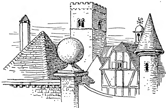
USE OF ELEMENTARY FORMS IN ARCHITECTURE.
